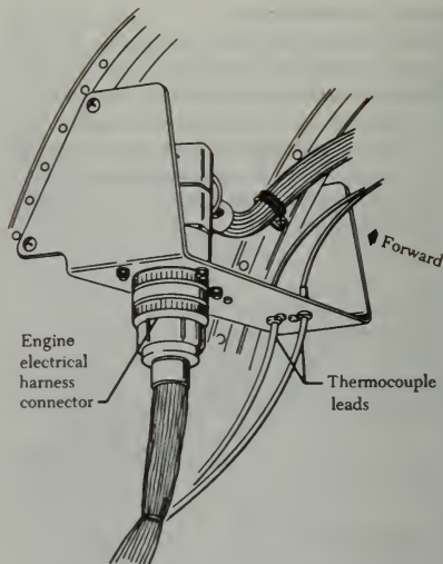
FIGURE 8-16. Electrical disconnect.
